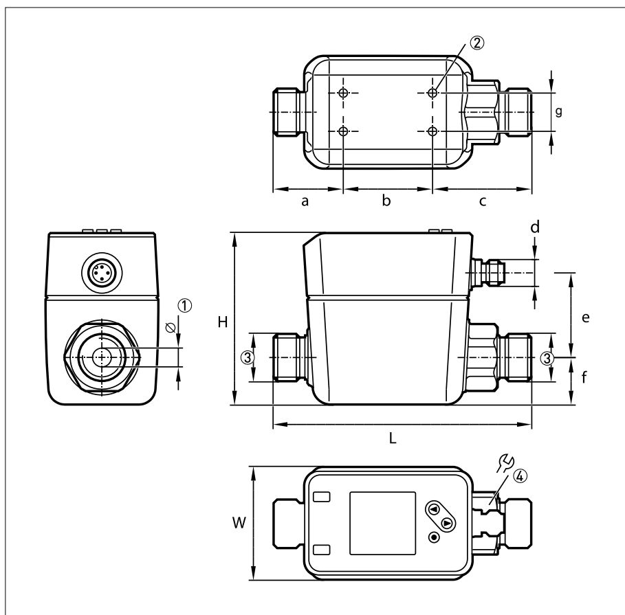
Figure 2-1: 寸法 [mm]
